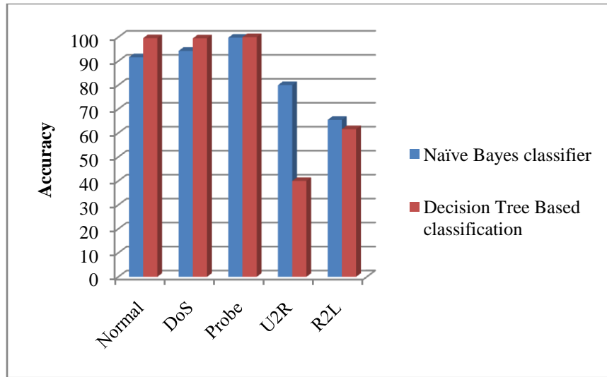
Figure 1: Accuracy comparison graph by using training data set
